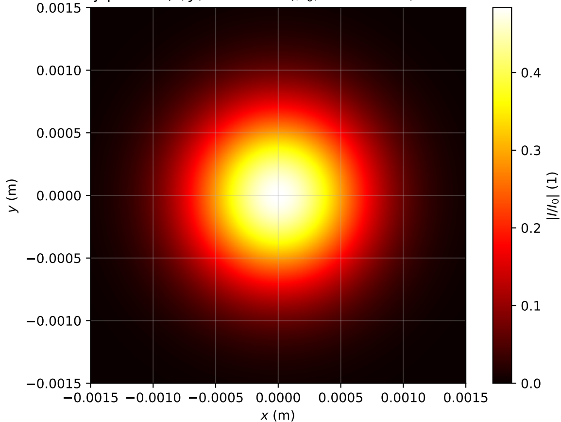
Intensity profile I(x, y, z = 2.229m)/I_0 , Pin=0.1Pcr, artificial time
